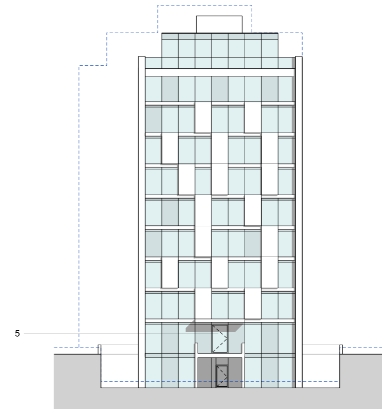
North Elevation (facing square) BUILDING E
