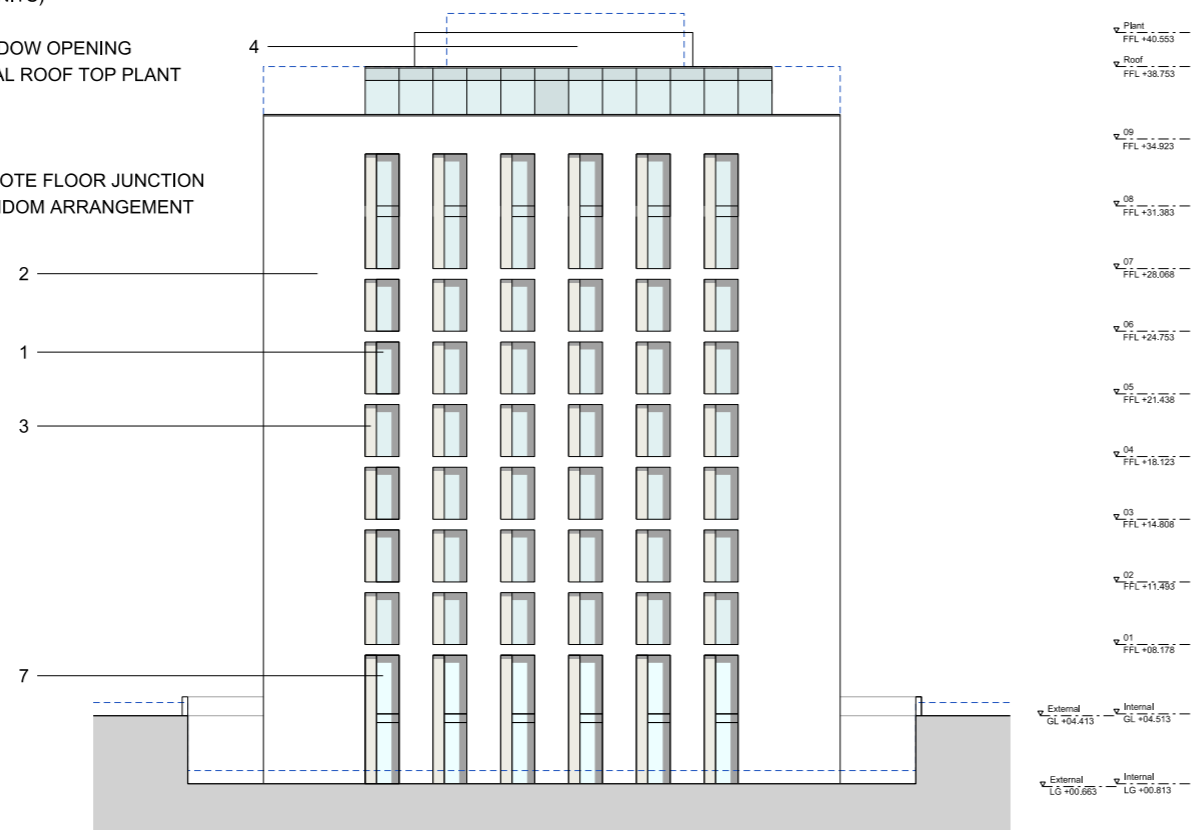
West Elevation BUILDING E
