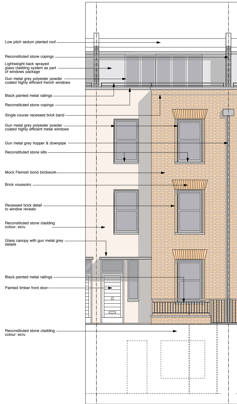
Type A - front elevation (west)
