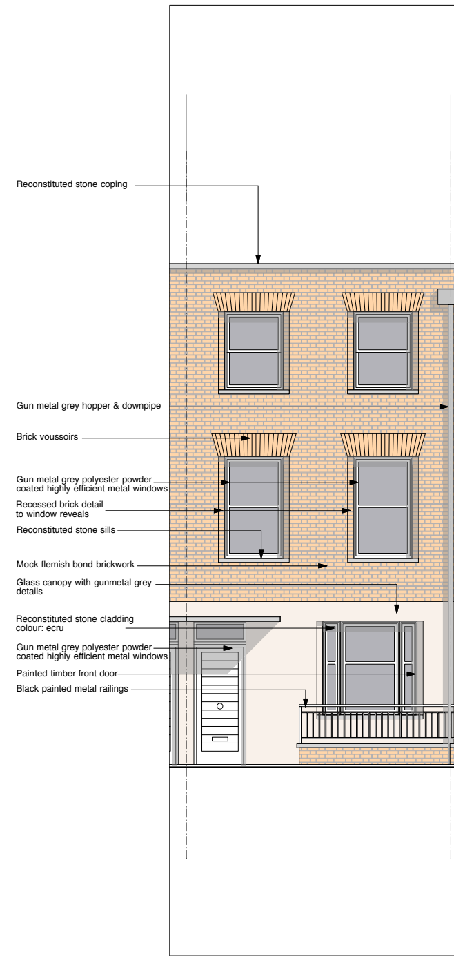
Type C - front elevation (west)
