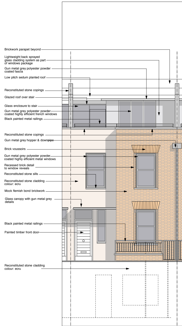
Type B - front elevation (west)
