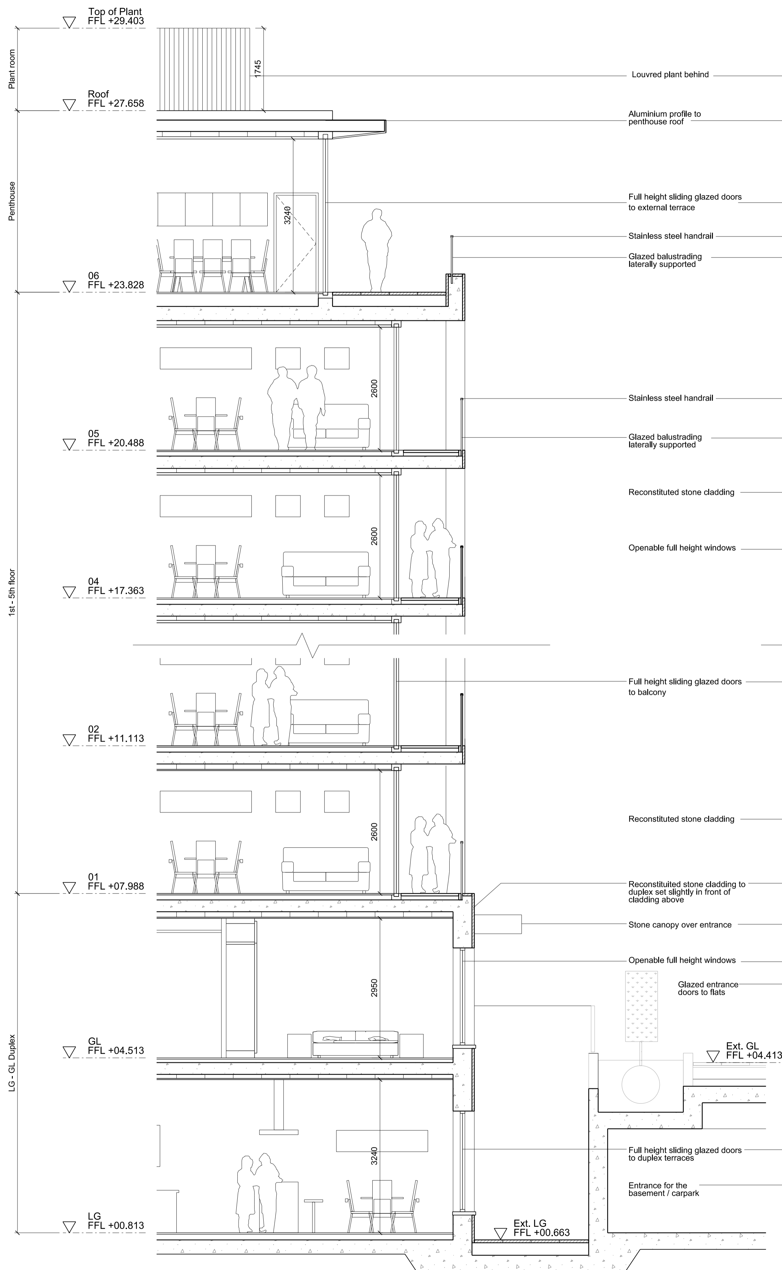
A Wall section BUILDING F
