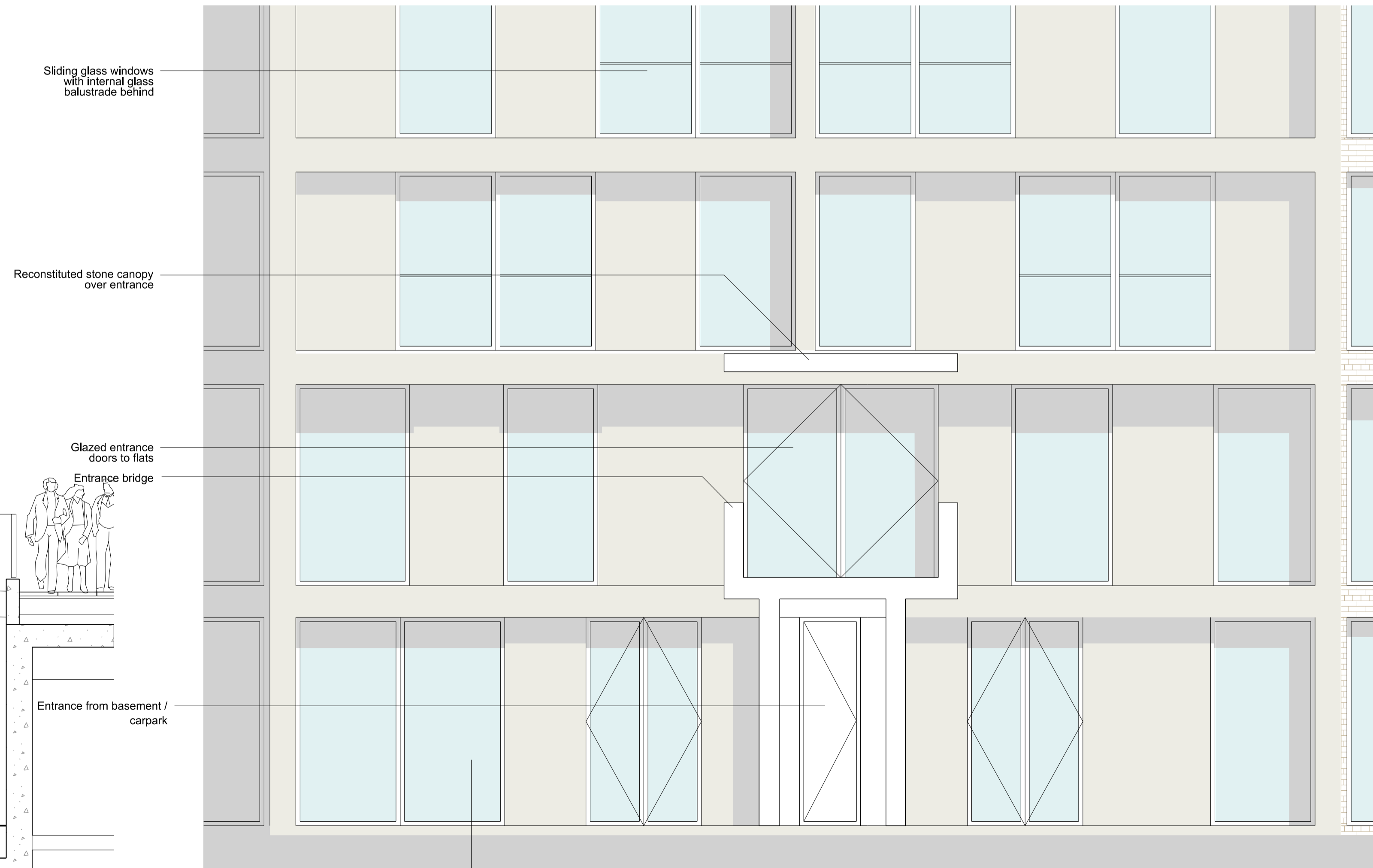
A West Elevation Typical Bay BUILDING C
