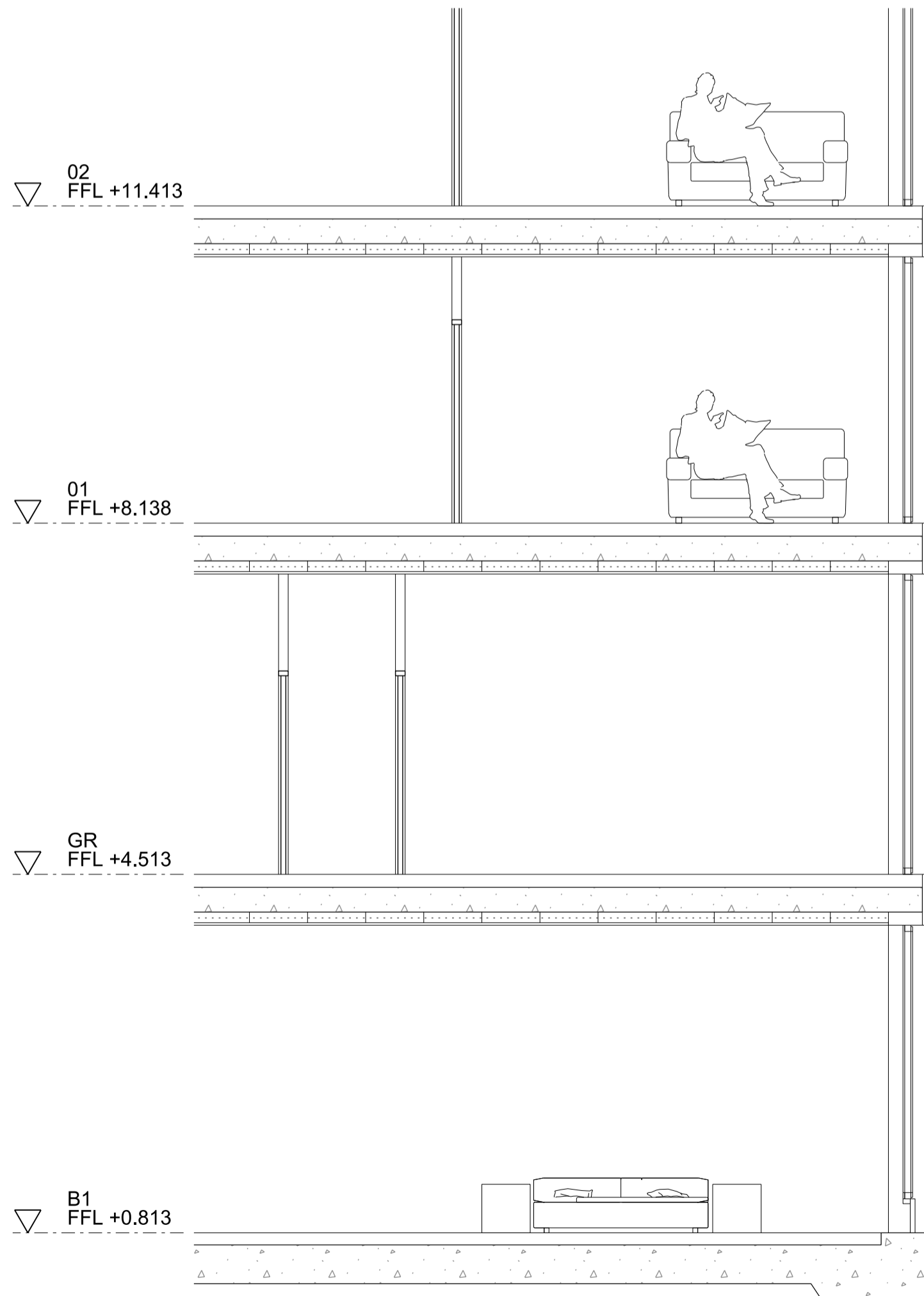
A Section through West Elevation BUILDING C
