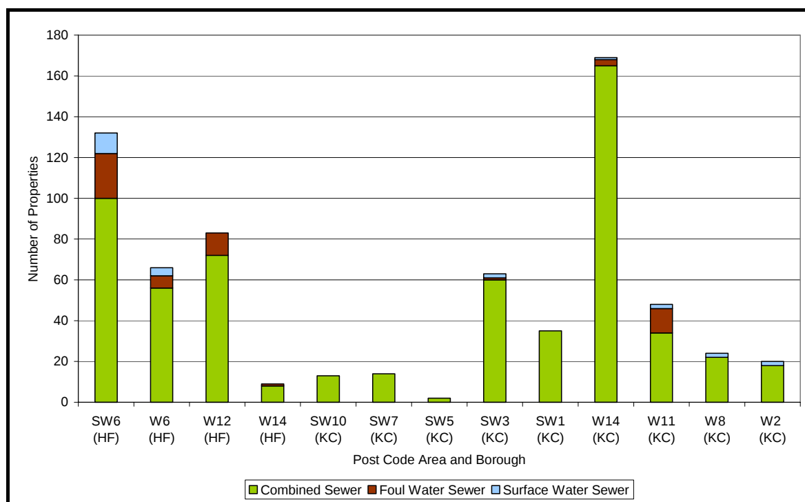
Figure 4.1: Total Number of Properties Flooded by Overloaded Sewers in the last 10 years
