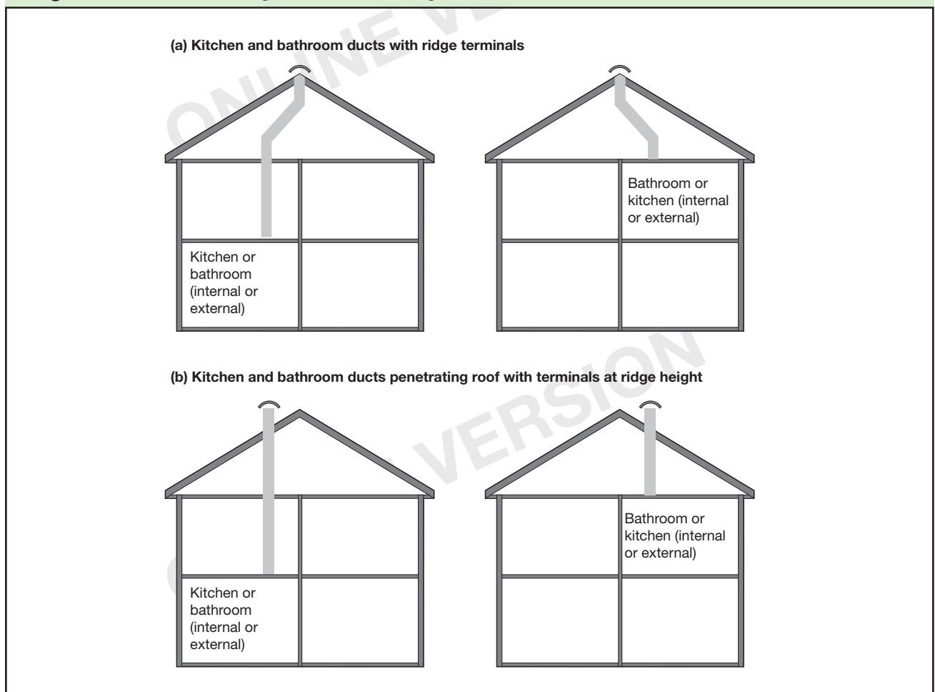
Diagram D1 Suitable layouts for PSV systems
