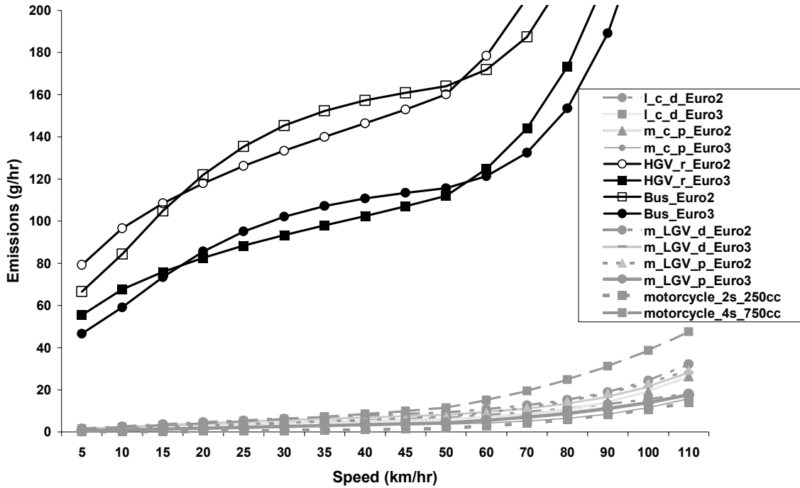
Figure 3 Emissions NO x (g/hr) for Euro 2 and 3 Vehicles at different Average Speeds (km/hr)
