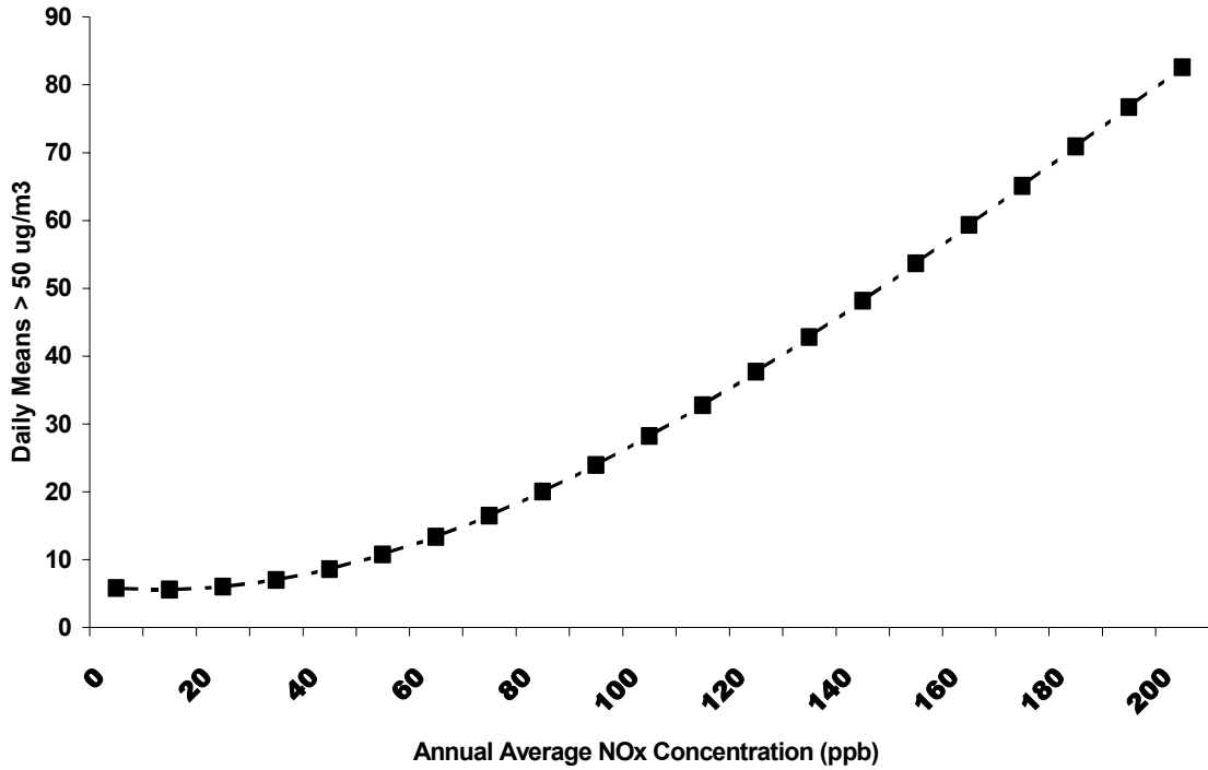
Figure 2 The relationship between annual mean NO x and days where PM10 > 50 µg/m 3
