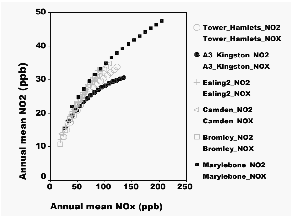
Figure 1 NO x and NO 2 Relationships at Roadside Sites across London (1999)
